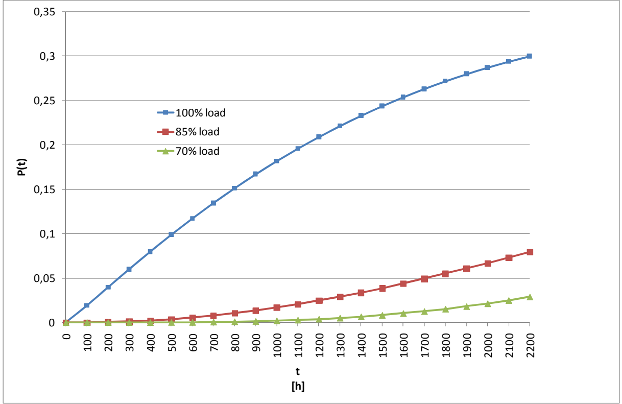
Fig. 4 Occurrence probability of the number k' of the events N_{\Delta gp} in function of considered engine load values and engine use duration period
