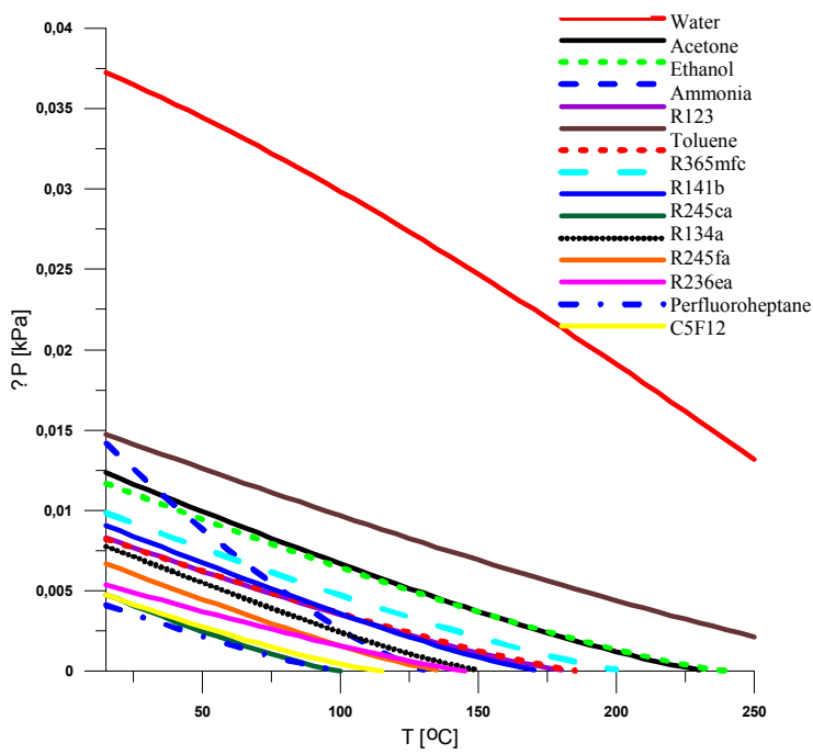
Fig. 2b. Effect of capillary pressure rise pressure on the temperature for different working fluids (for the assumed contact angle of liquid equal to 70^{\circ} )
