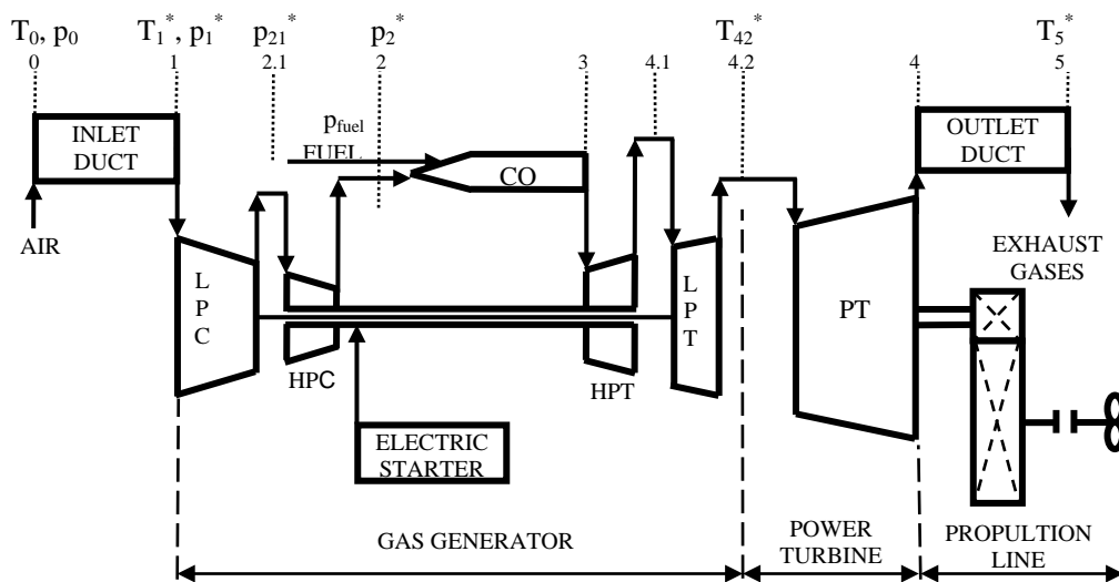
Fig. 2. Block diagram of DR77 gas turbine engine
