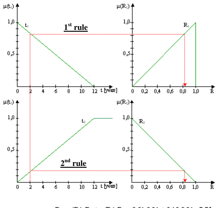
Fig. 2. Reliability of galvanized steel pipeline for two years period of time assessed with fuzzy inference methods
