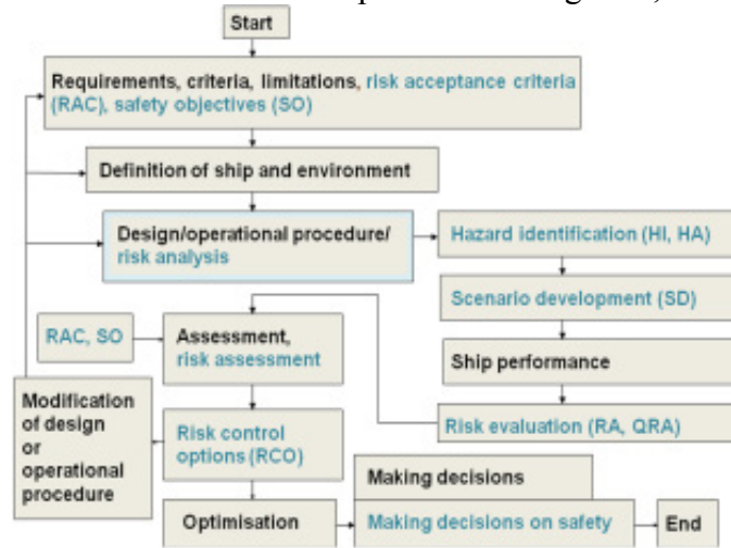
Figure 2. Structure of the method of risk and safety assessment of ships in damaged conditions.
