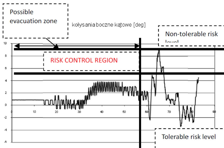
Figure 5. An example of the roll function in time domain and risk evaluation criteria applied for the assessment of safety of the container ship in abnormal/damaged conditions.
