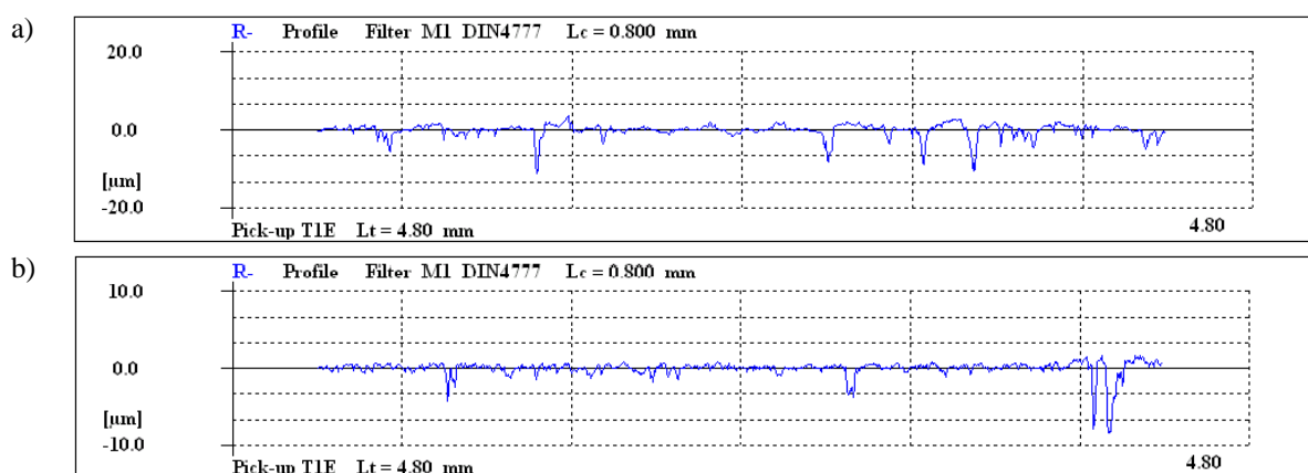
Fig. 4. Examples of roughness profiles of Ni-Al-15%Al 2 O 3 coatings obtained by plasma spraying: a) the turned ( R_a = 1.02 \mu\text{m} ), b) the burnished ( R_a = 0.71 \mu\text{m} ),
