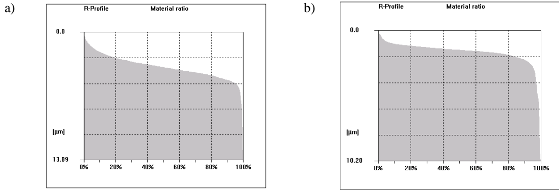
Fig. 5. Examples of material ratio curves of the surface Ni-Al-15%Al 2 O 3 coatings obtained by plasma spraying: a) the turned, b) the burnished
