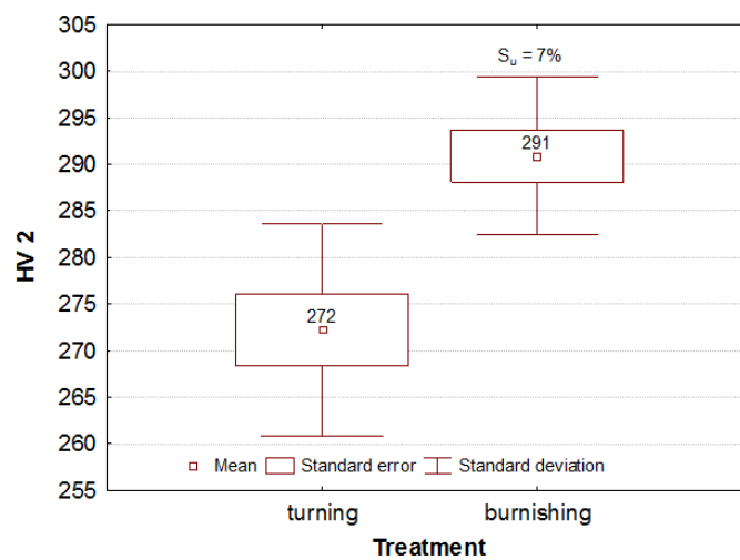
Fig. 7. Effect of treatment on hardness and relative degree of strain hardening ( S_u ) of surface Ni-Al-15%Al 2 O 3 coatings
