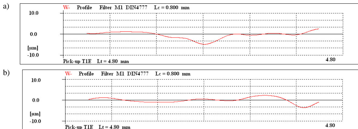
Fig. 3. Examples of waviness profiles of Ni-Al-15%Al 2 O 3 coatings obtained by plasma spraying: a) the turned ( W_t = 7.41 \mu\text{m} ), b) the burnished ( W_t = 7.13 \mu\text{m} ),
